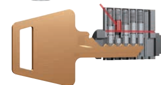
Reverse rake tapered driver pin
