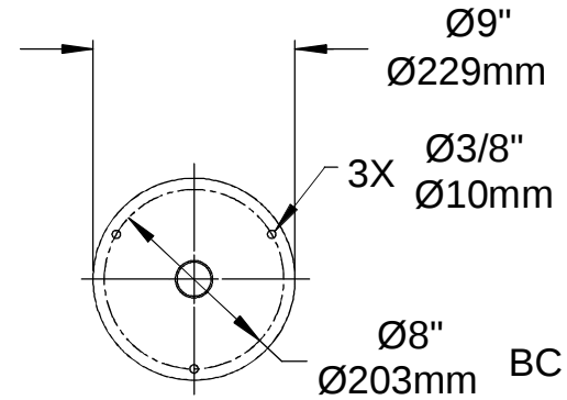
MOUNTING DETAIL
