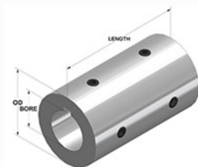
Metric Set Screw Coupling with Keyway 4-Holes
