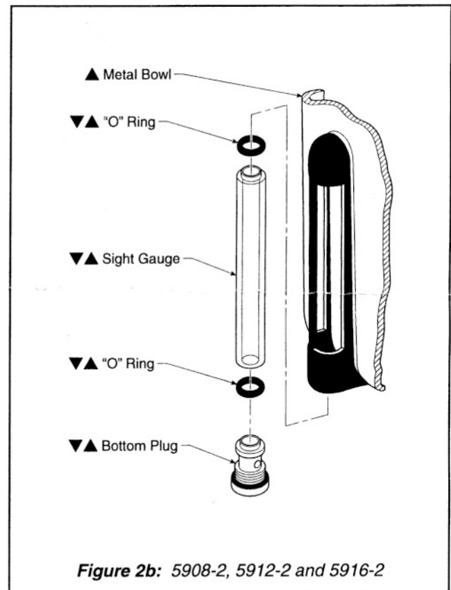
Figure 2: Lubricator Parts
